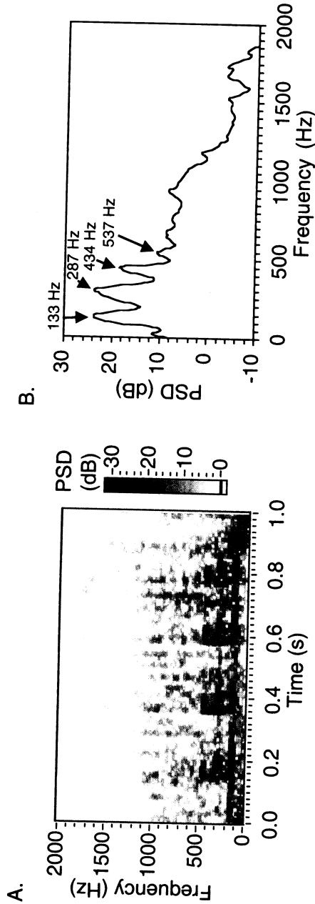
FIG. 12. A) Sonogram of red drum "drum", slide factor: 128 samples, recorded 17 September 1997 at station 5. B) Average power spectrum taken from 0.133 to 0.848 sec in the recording (16 consecutive power spectra). Peaks in the power spectrum occurred at 133, 287 and 434 Hz. The dominant frequency was 287 Hz, although the peak at 133 Hz was almost as large. A very small maximum occurred at 537 Hz.
